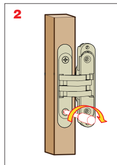
2 Mounting of fixed base and of hinge in the door; flat countersunk-head self-tapping screw
