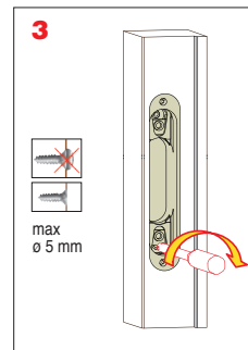
3 Mounting of fixed base and of hinge in the door; flat countersunk-head self-tapping screw
