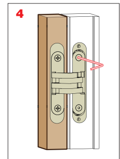
4 Mounting of hinge in the post; countersunk-head screw, allen screw included in the kit
