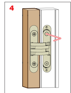
Mounting of hinge in the post; countersunk-head screw, allen screw included in the kit
