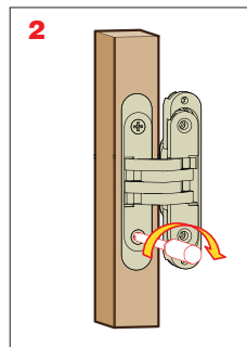
Mounting of fixed base and of hinge in the door; flat countersunk-head self-tapping screw
