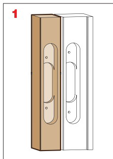
Hollows execution in the door and in the post
