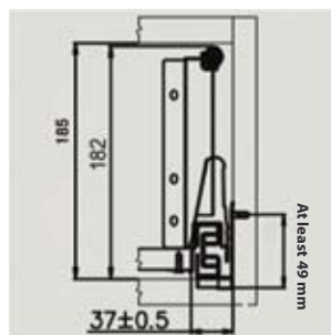
Installation of front fixing brackets
