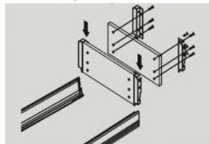
Railing installation
