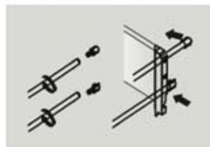
Installation of drawer
