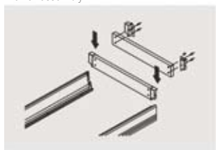
Drawer assembly
