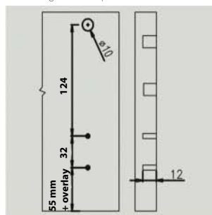
Removal of front panel
