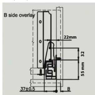
Front panel position
