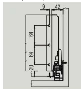
Back fixing brackets position
