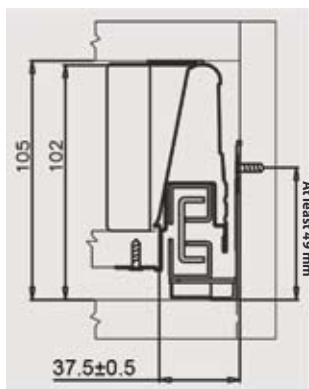
Cabinet dimension
