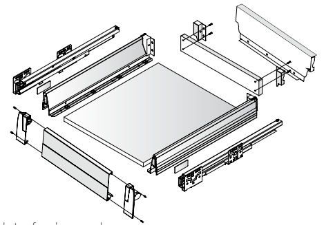
Front plate for inner drawer
