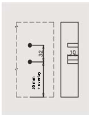
Front fixing brackets position
