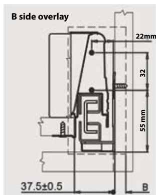
Front panel position
