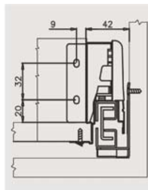
Back fixing brackets position
