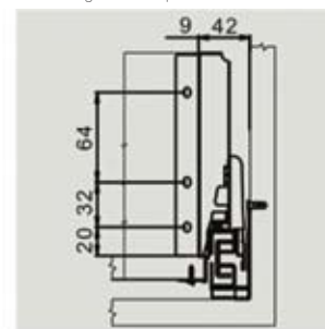
Back fixing brackets position
