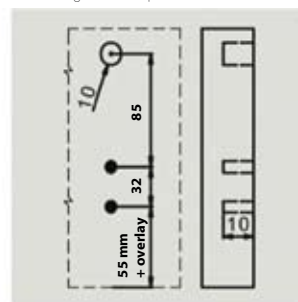
Front fixing brackets position
