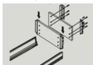
Railing installation
