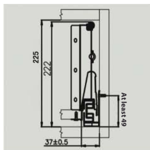
Installation of front fixing brackets
